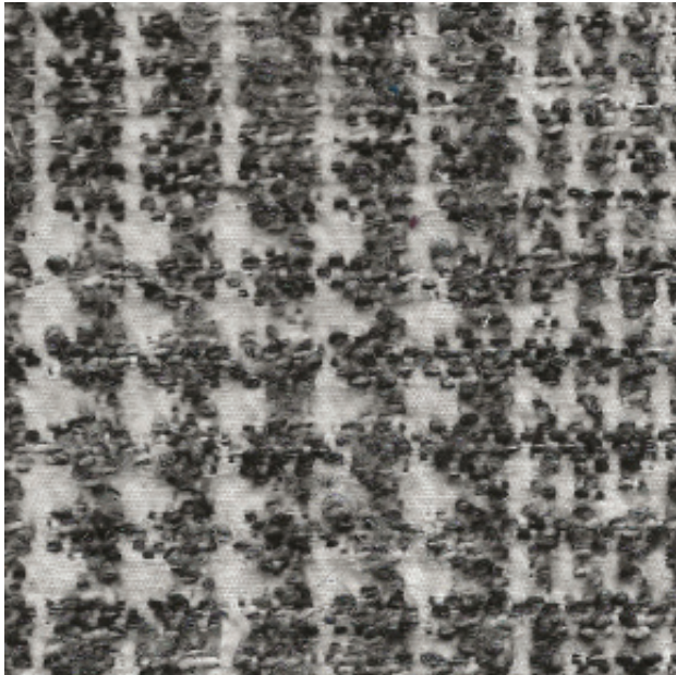
01 Payne
